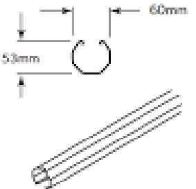
LYSAGHT® FENCE RAIL
